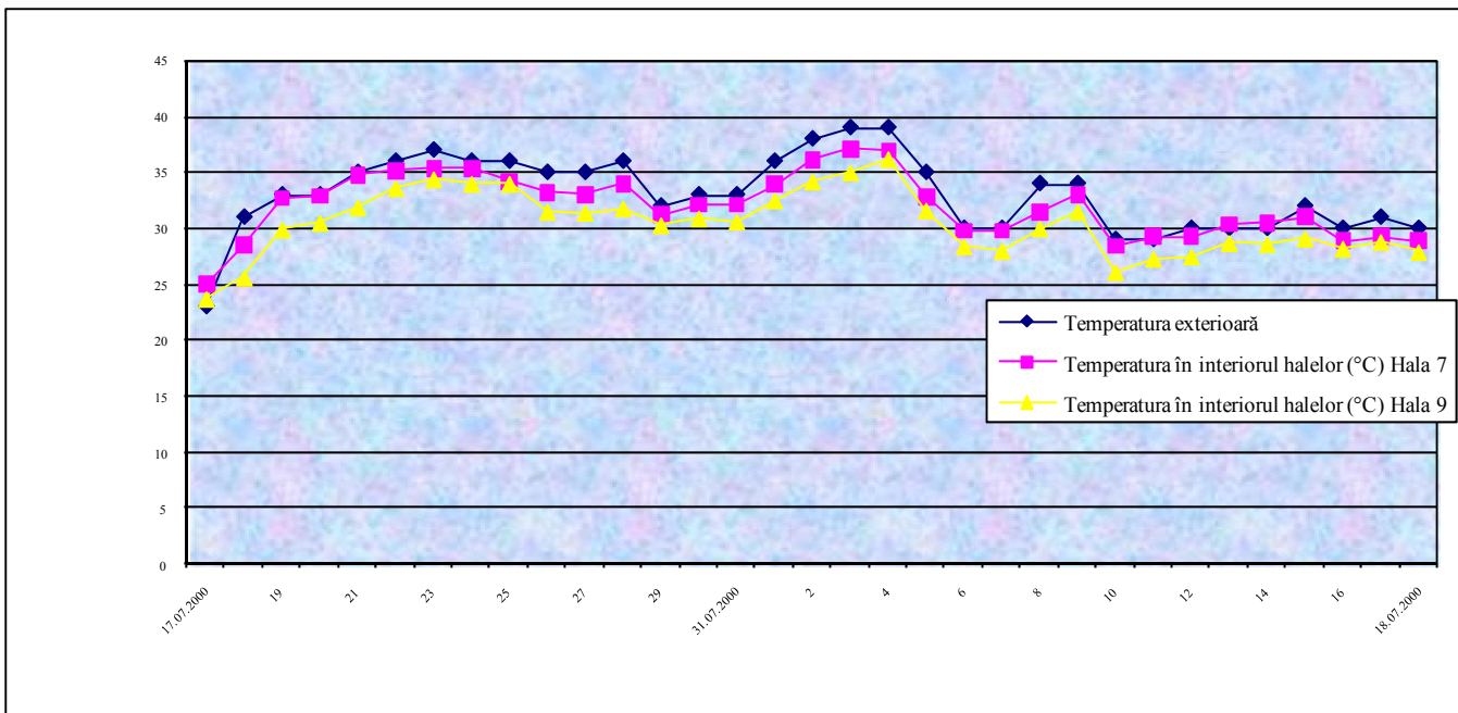
Fig. 3 Evolution of temperature inside the hall 7 and Hall 9 depending on the temperature outside
