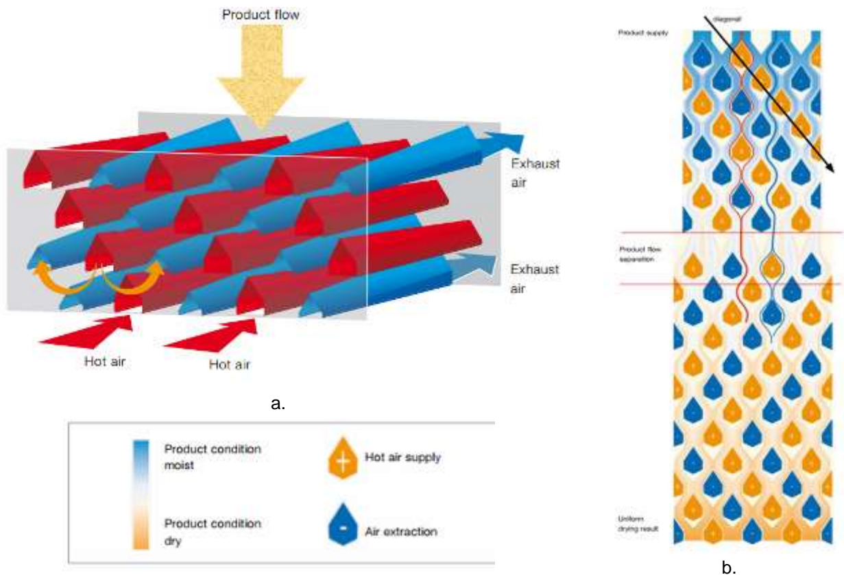
Fig. 8 – Scheme of drying column of Eco Dry dryers [14] a. airflow through conical pipes; b. Layout of pipelines
