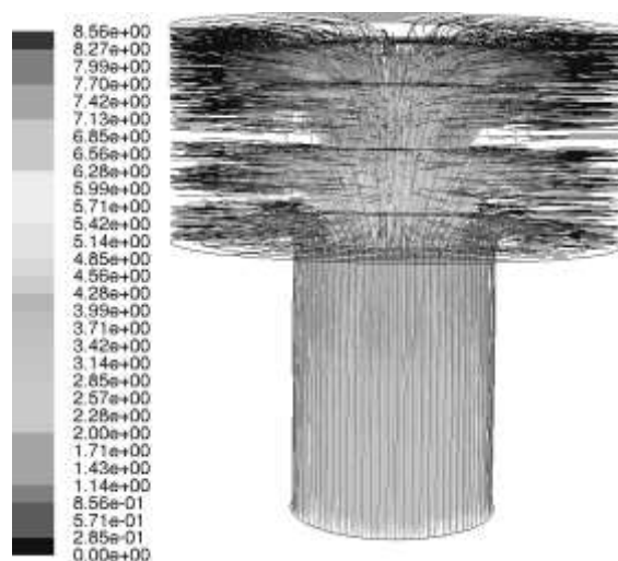
Figure 9 The pathlines field inside the dryer with baffles and three layers v (m/s) (dryer temperature of 70 °C)
