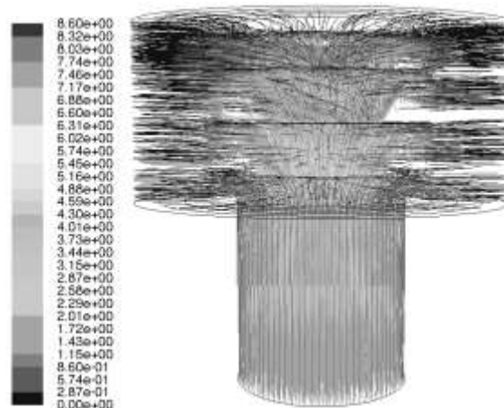
Figure 8 The pathlines field inside the dryer with baffles and three layers v (m/s) (dryer temperature of 40 °C)
