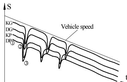
Figura 1a Variation of speed in relation to the braking time
