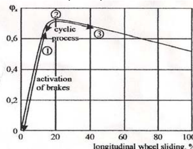
Figura 1b The response of the coefficient of cohesion of tyres with the surface of the road
