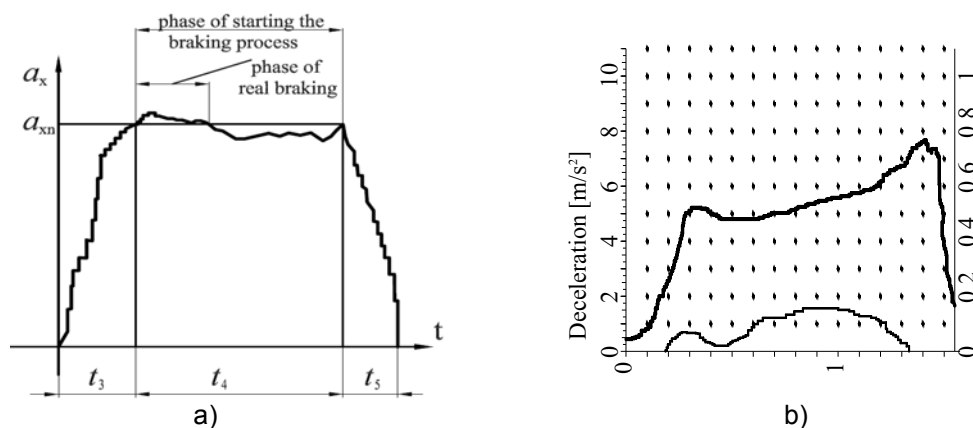
Figura 4 Diagram of braking without ABS a) phase of starting the braking process b) phase of real braking
