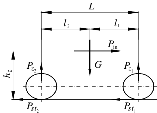
Figura 2 Scheme of forces in the process of braking without wheels blocking
