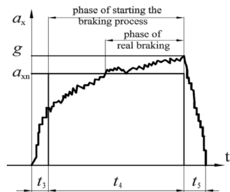
Figura 3 Diagram of braking with ABS-phase of starting the braking process
